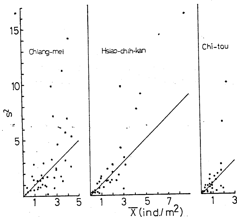
Fig. 6. The relationship between the mean and mean square of G. tumidum density estimated in each plot.
