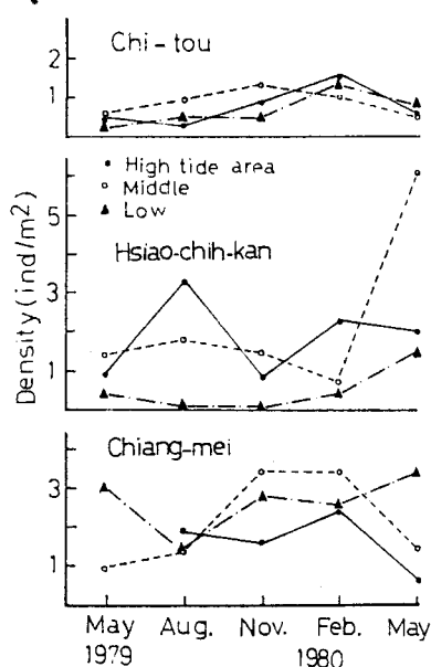
Fig. 7. Seasonal fluctuation of G. tumidum densities at three investigated areas.
