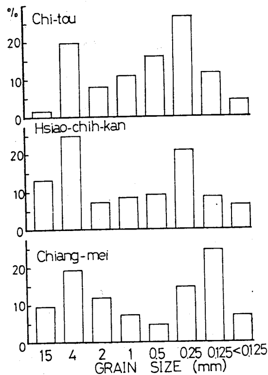
Fig. 2. Percentage composition (by weight) of substrate samples.
