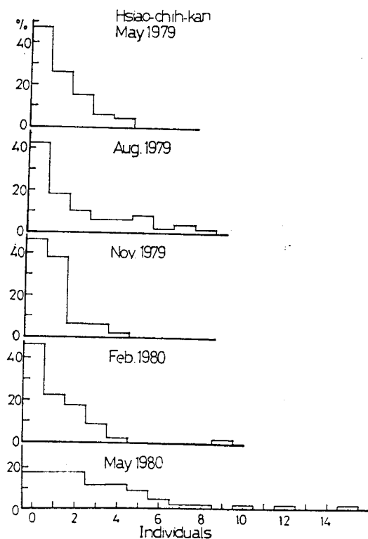
Fig. 3. Relative frequency distribution of individuals of G. tumidum collected in each plot at Hsiao-Chih-Kan
