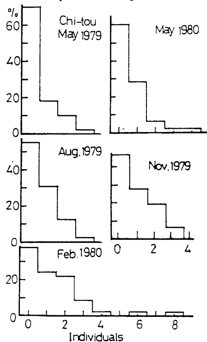
Fig. 5. Relative frequency distribution of individuals of G. tumidum collected in each plot at Chi-Tou.
