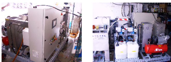
Fig. 2 Photos of the pilot-scale pulsed electrocoagulation treatment system.
