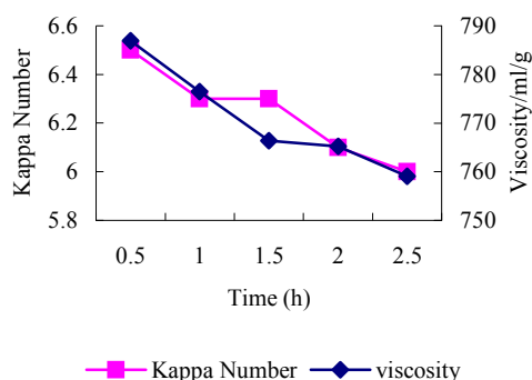
Fig. 2 Effect of oxygen delignification with xylanase post-treatment conditions: pH 6.0, temperature 50°C, pulp consistency
