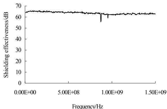
Fig. 5 Electromagnetic shielding effectiveness of the plated birch veneer.
