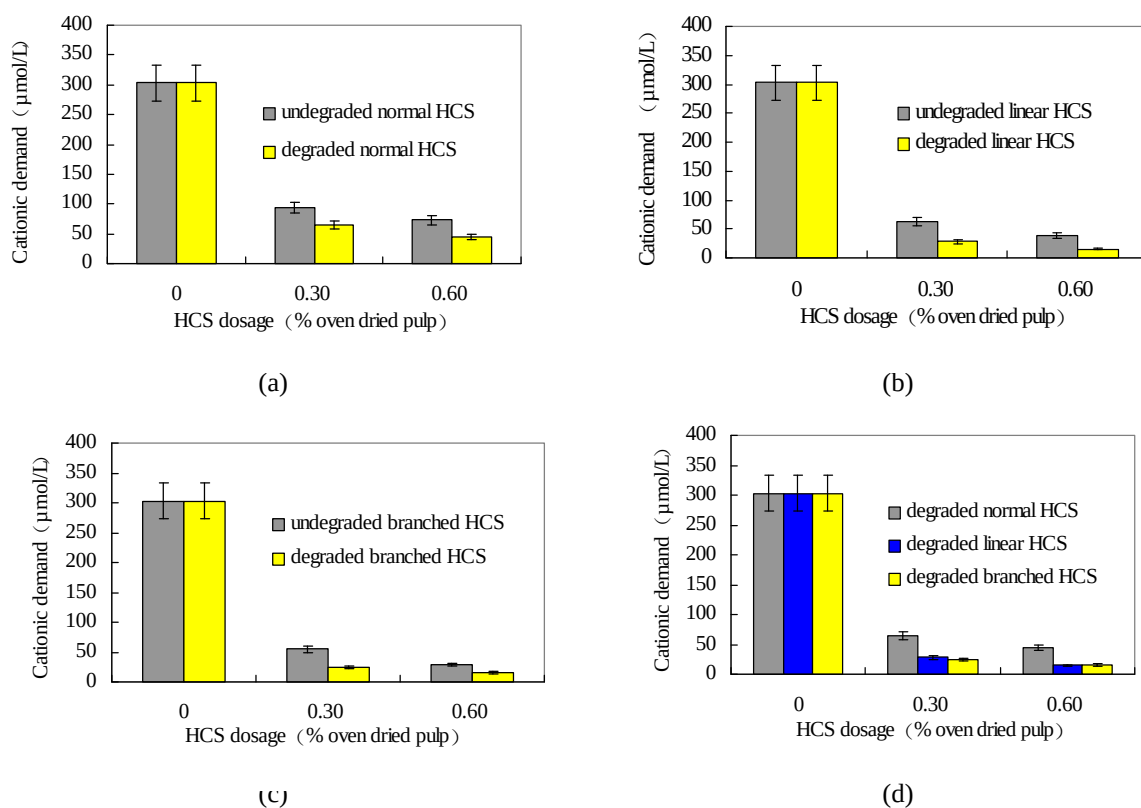
Figure 3 Effects of HCSs with different branching degrees and molecular weights on cationic demand of filtrate (The cationic demands were measured with a Mutek PCD 03 Particle Charge Detector from BTG Group, Sweden. Both the degraded and undegraded HCSs decreased the cationic demands of the deinked pulp, and the degraded HCSs showed better performance than their corresponding undegraded ones)
