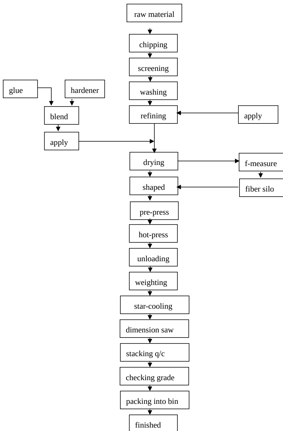
50, 000m 3 /a Cont-roller MDF line process flowchart
