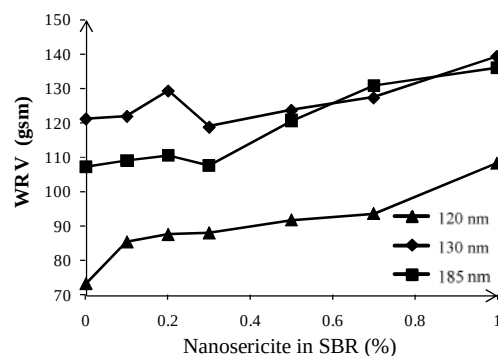
Fig. 2. Effects of nanosericite proportion and SBR particle size on the water retention value.
