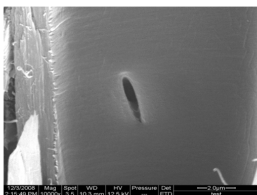
Fig. 2 Untreated fiber tracheid with smooth and undamaged S3 layer.
