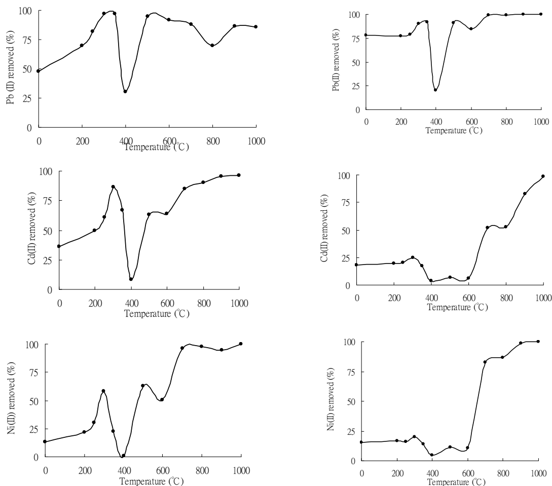
Fig. 1 Effects of thermal modification on metal-removal ability of Phyllostachys pubescens wastes.
