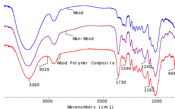
Fig. 2 FTIR spectra of wood and the two types of wood composites.
