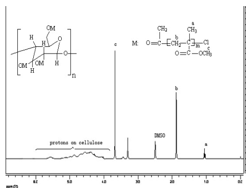
Figure 3 ^1\text{H} NMR of Cell-PMMA in \text{DMSO}-d_6
