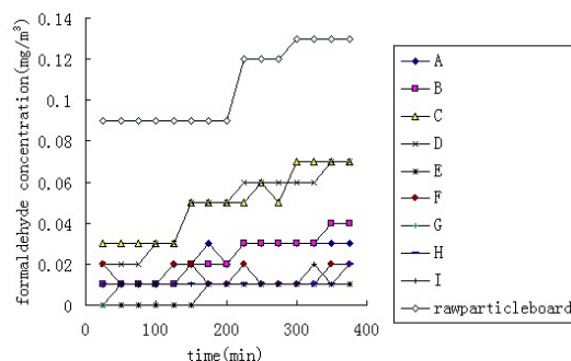
Fig. 4 Formaldehyde emission concentration measured in 6 hours.
