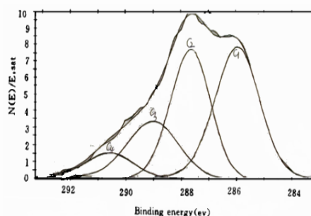
Fig. 4 C1s spectra of treated wood.
