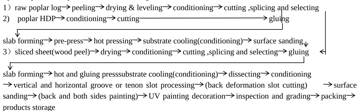
Fig. 4 The “overlap together and gluing press twice” process of Multi-layer wood floorings use poplar veneer & HDP as substrate.
