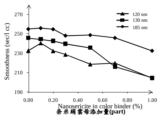
Fig. 8. Effects of nanosericite and SBR particlesize on the coated paper Smoothness.
