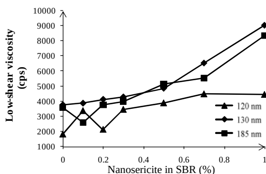
Fig. 3. Effects of nanosericite proportion and SBR particle size on the low-shear viscosity of SBR.
