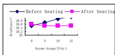
Fig. 4 Effect of before and after beating on Brightness
