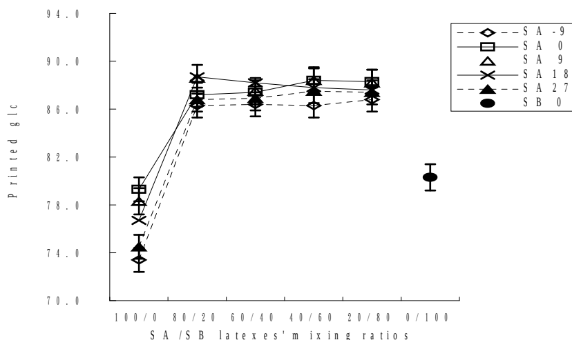
Fig. 5 Effects of SA_{250} 's Tg and ratio with SB_{100} on the printed gloss of LWC.
