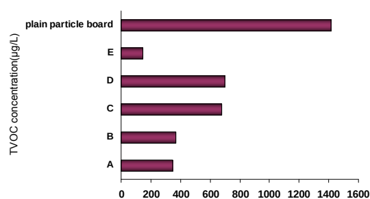
Fig. 2 TVOC emission concentration measured after 1d.
