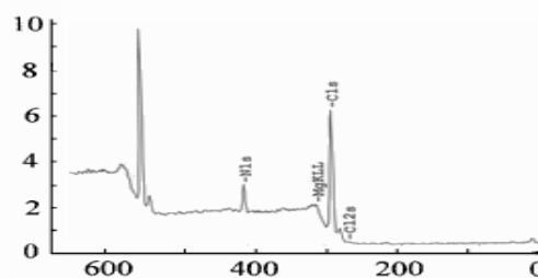
Fig. 2 XPS spectra of treated wood surface.
