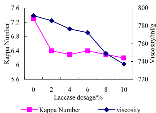
Fig. 3 Effect of X dosage during post-treatment treatment conditions: pH 6.0, temperature 50°C, pulp consistency 5% and treated for 1 hour.
