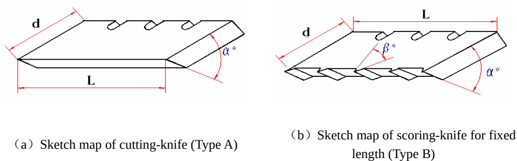
Fig. 3 The two types knives sketch map of BOSB Flaker.
