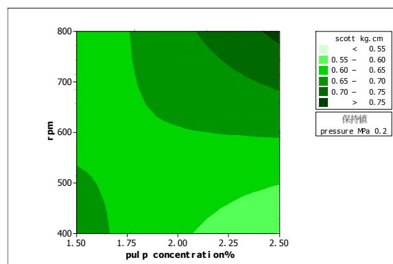
Fig.5 contour plot of Z-bond vs rotate speed &amp; pulp concentration
