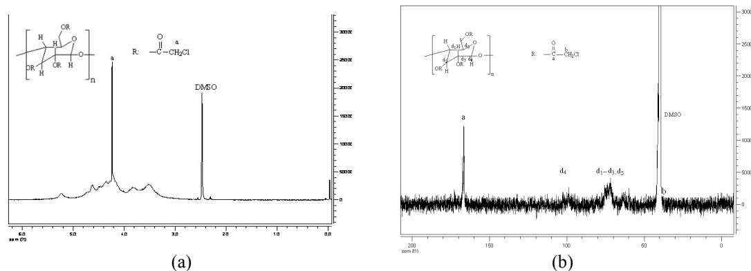
Figure 2 ^1\text{H} NMR (a) and ^{13}\text{C} NMR (b) spectra of Cell-AcCl (DS = 1.87) in \text{DMSO}-d_6 .
