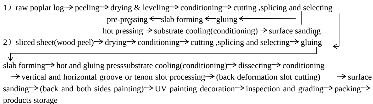
Fig. 3 The “overlap together and gluing press twice” process of Multi-layer wood floorings use poplar veneer as substrate.
