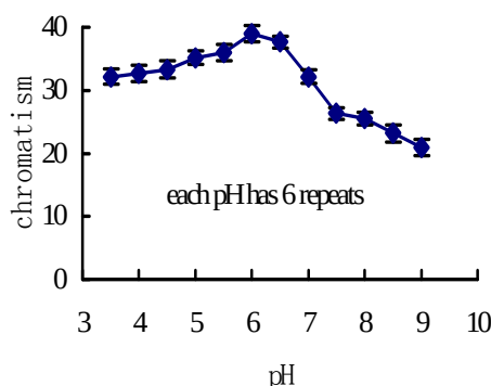
Fig. 1 pH-Chromatism curve.
