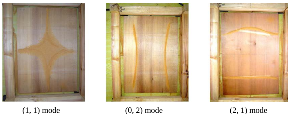
Fig. 1 Chladni patterns of different vibration modes.
