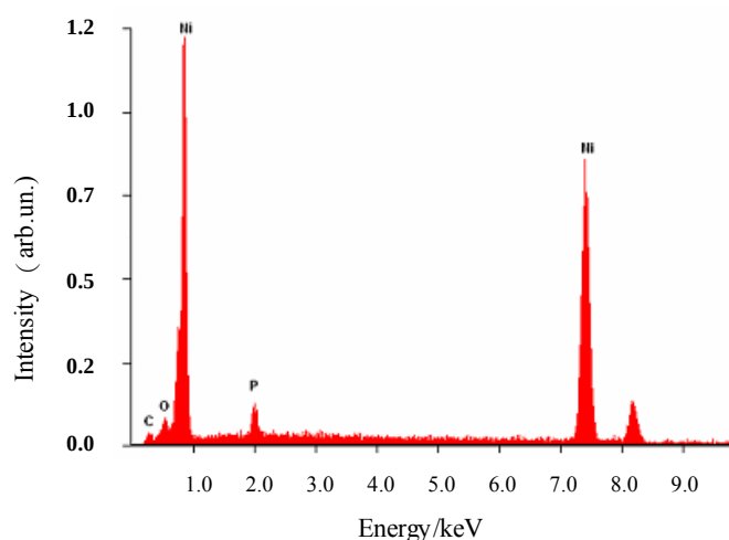
Fig. 3 EDS spectrum of the plated birch veneer.
