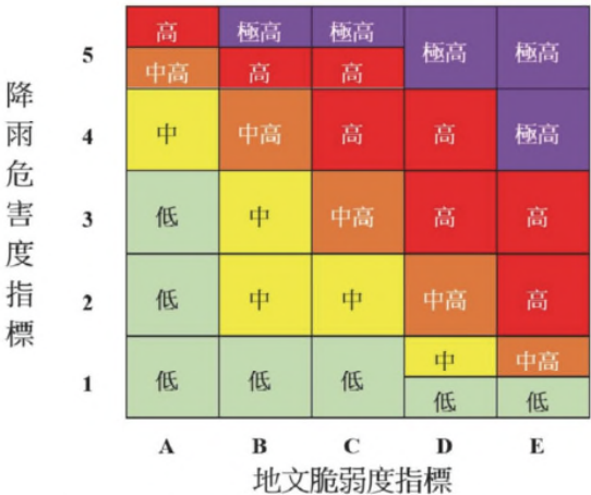
圖 6 以矩陣法定義之降雨致災風險等級指標 ( R_h ) Fig.6 The definition of risk level of rainfall-induced hazard ( R_h ) by matrix
