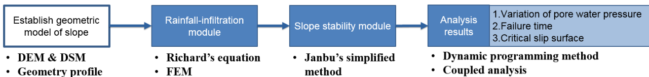
Fig. 1 The operating procedure of Integrated Rainfall Infiltration Slope stability (IRIS) model.
