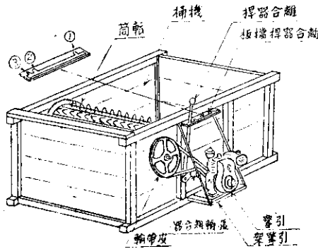
(圖造構機谷脫力動易簡)
